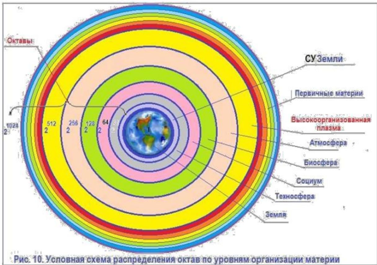
Fig. 10. Conditional scheme of the distribution of octaves on the levels of the organization of matter
